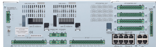
VX-3016F rear
