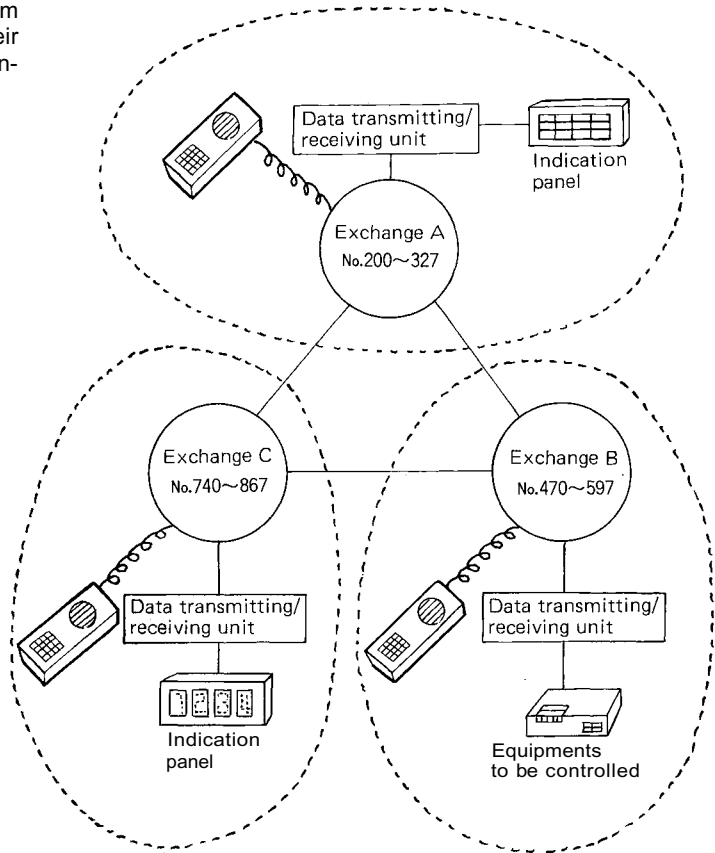
Control of Data Transmitting and Receiving Units of each exchange is only possible from the stations sharing the same exchange and within the same areas circled in dotted lines.
